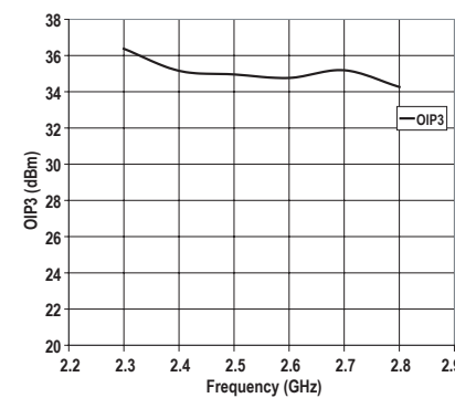
Figure 27. OIP3 vs Frequency
