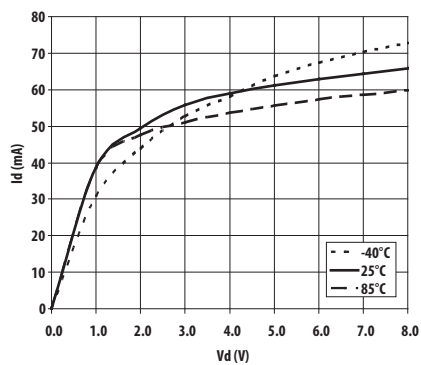
Figure 11. I_d Vs V_d and Temperature
