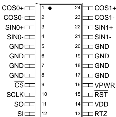
Figure 3. 33976 Pin Connections
