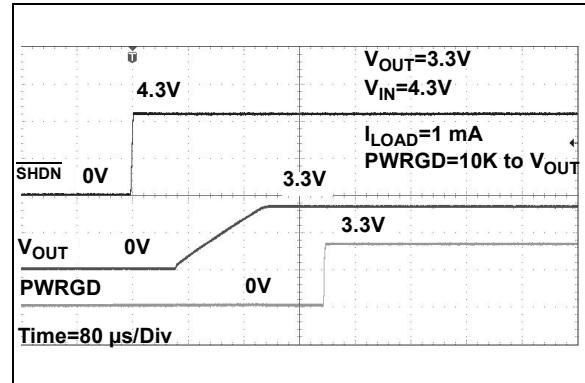
FIGURE 2-28: Start-up from \overline{\text{SHDN}} .
