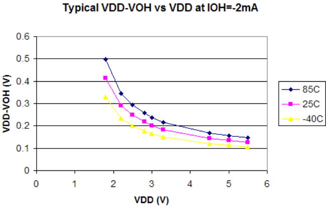
Figure 12-13. Typical V_{DD}-V_{OH} vs. V_{DD} at I_{OH}=2mA
