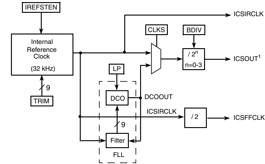
Figure 9-2. Internal Clock Source (ICS) Block Diagram
