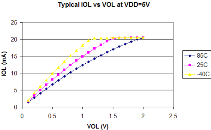
Figure 12-11. Typical I_{OL} vs. V_{OL} V_{DD} = 5 V
