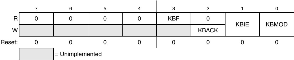
Figure 7-3. KBI Status and Control Register (KBISC)
