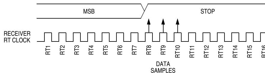
Figure 15-8. Slow Data
