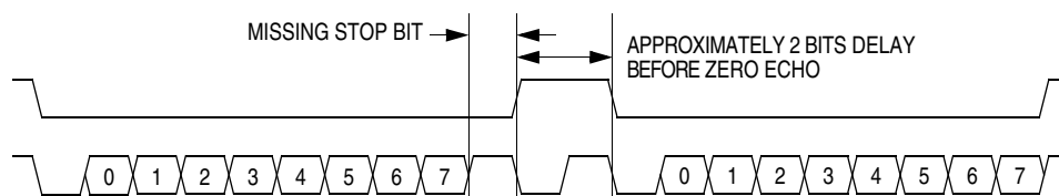
Figure 20-12. Break Transaction
