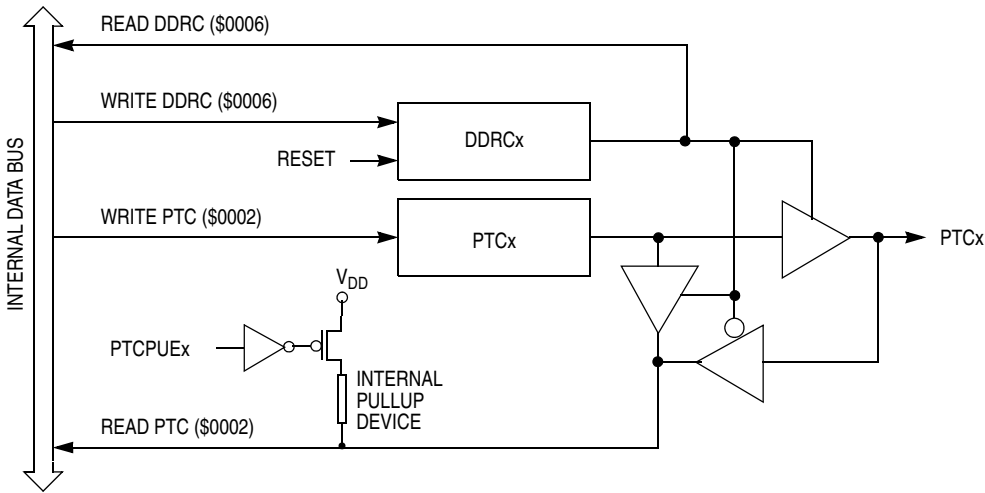
Figure 13-11. Port C I/O Circuit
