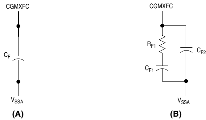
Figure 4-9. PLL Filter
