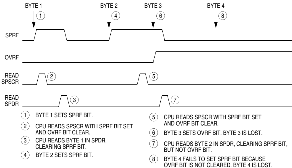
Figure 17-10. Missed Read of Overflow Condition
