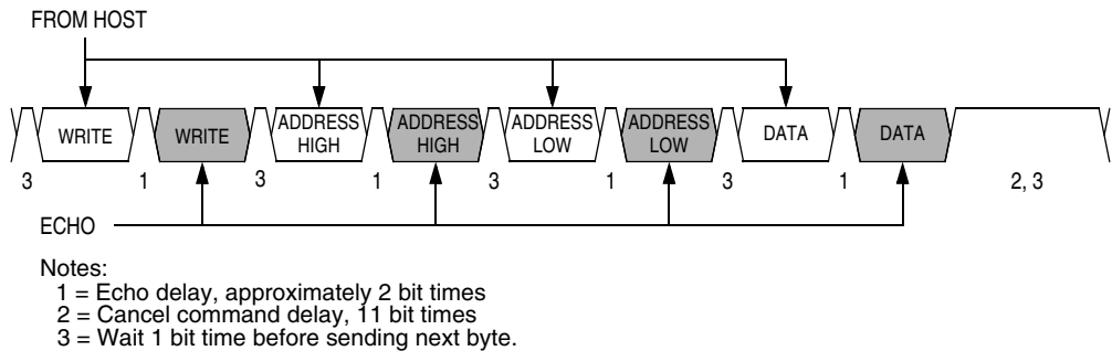
Figure 20-14. Write Transaction
