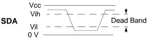
Figure 12. SDA/SCL Levels
