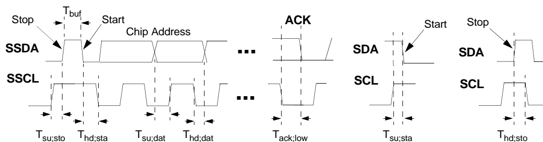
Figure 11. SSDA/SSCL Timing
