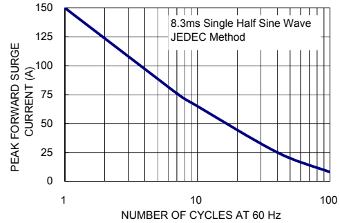
FIG. 2- MAXIMUM NON-REPETITIVE FORWARD SURGE CURRENT PER LEG
