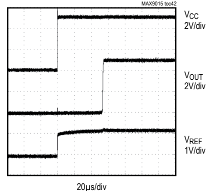
POWER-UP RESPONSE
