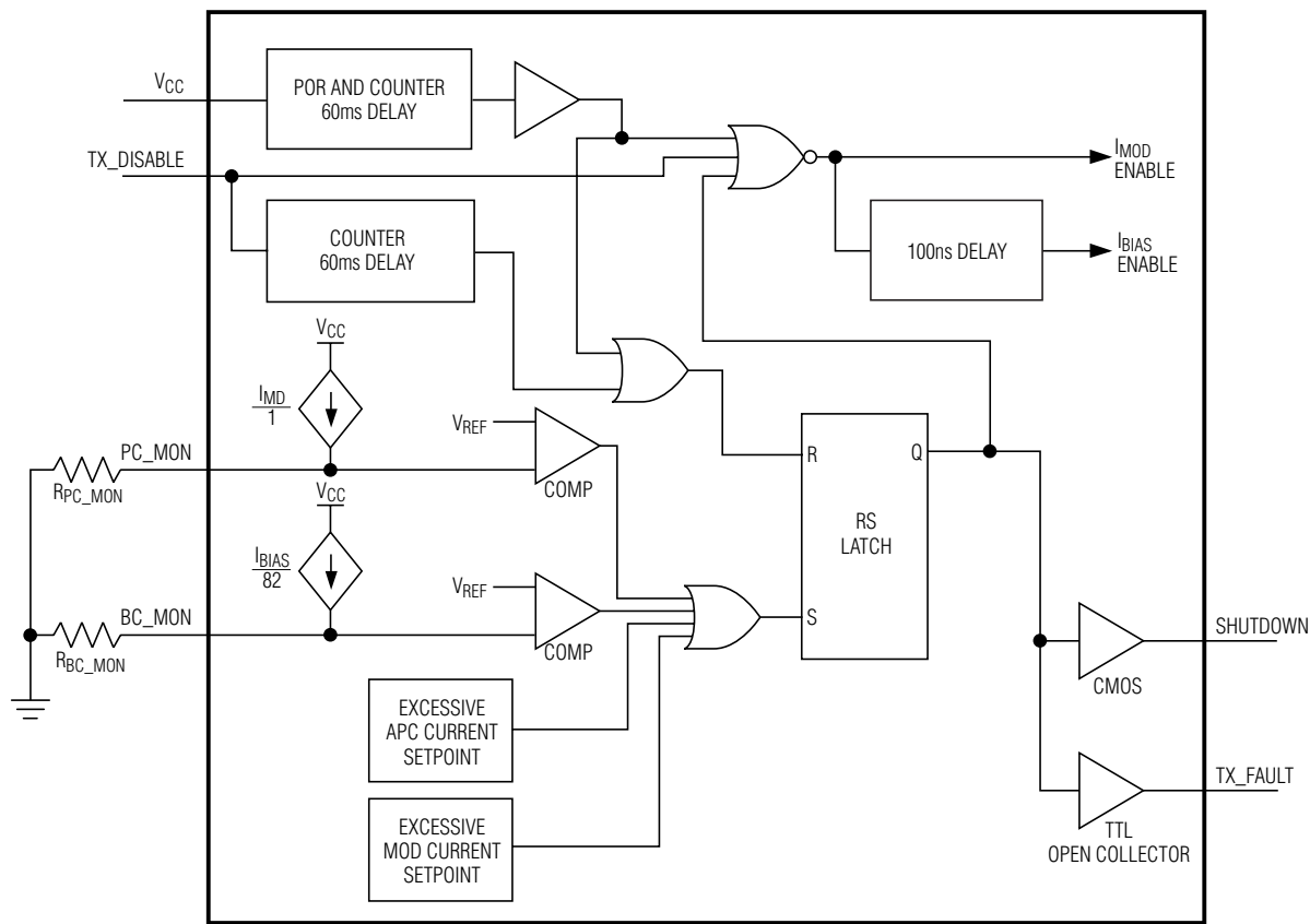
Figure 5. Simplified Safety Circuit
