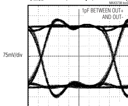
ELECTRICAL EYE DIAGRAM ( I_{MOD} = 30mA , 2.7Gbps, 2 7 - 1 PRBS)
