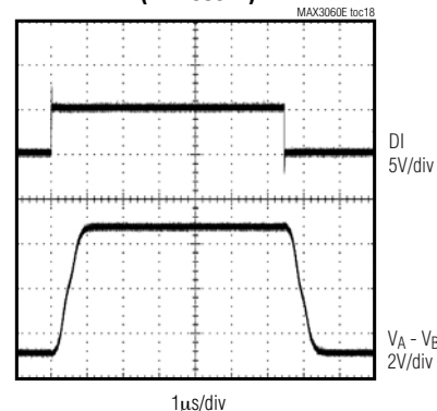
DRIVER PROPAGATION DELAY (MAX3061E)
