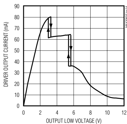
DRIVER OUTPUT CURRENT vs. OUTPUT LOW VOLTAGE
