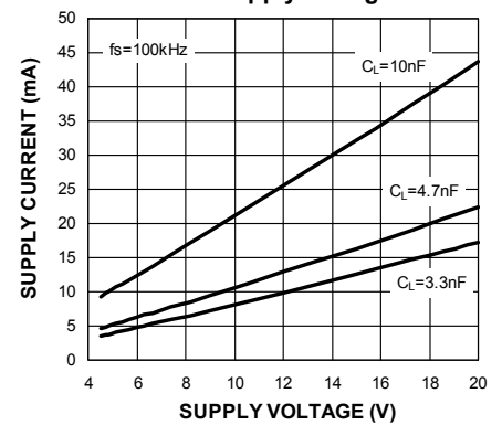
Supply Current ( I_S ) vs. Supply Voltage
