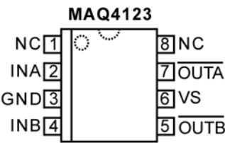
DUAL INVERTING
