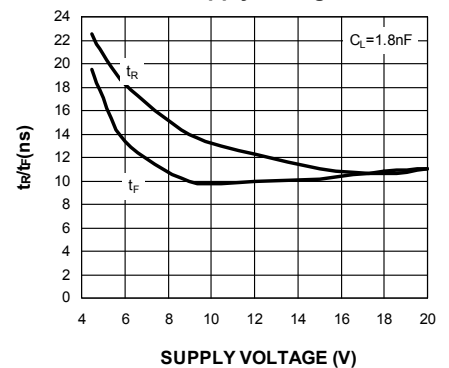
Output Rise/Fall Time vs. Supply Voltage
