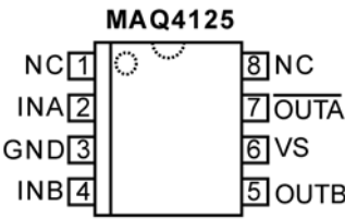
INVERTING + NON-INVERTING
