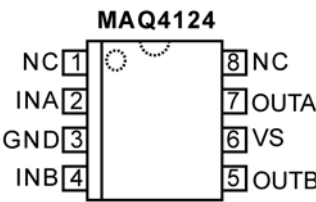
DUAL NON-INVERTING
