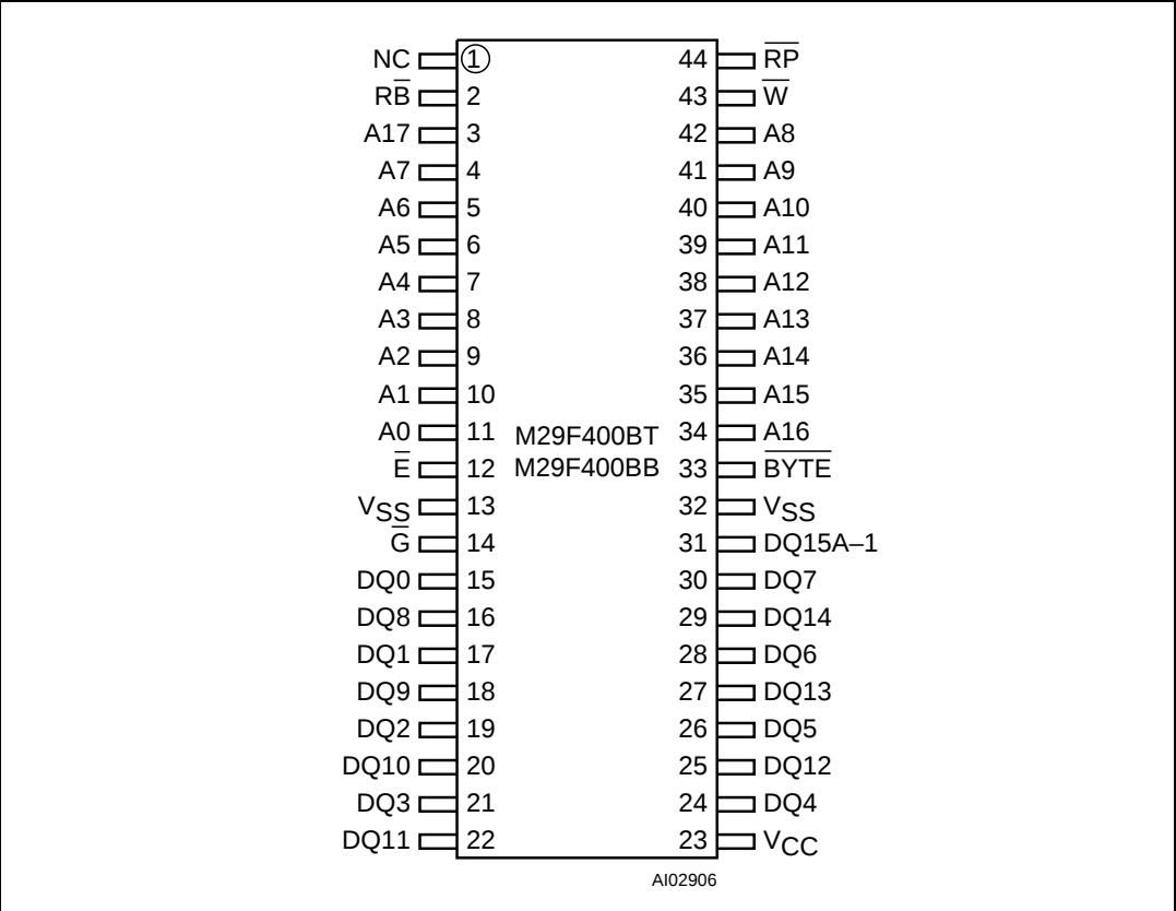
Figure 3. SO connections
