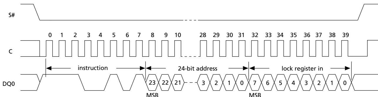
Figure 17: WRITE to LOCK REGISTER Instruction Sequence
