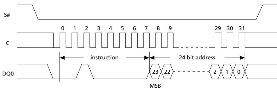
Figure 22: SUBSECTOR ERASE Command Sequence
