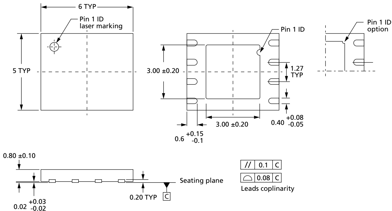
Figure 32: DFN8 6mm x 5mm
