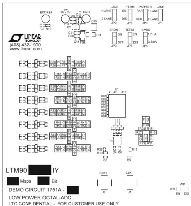
Silkscreen Top
