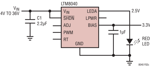
Figure 2c. Tie BIAS to an External Power Source if Neither V_{IN} Nor LPWR are Suitable
