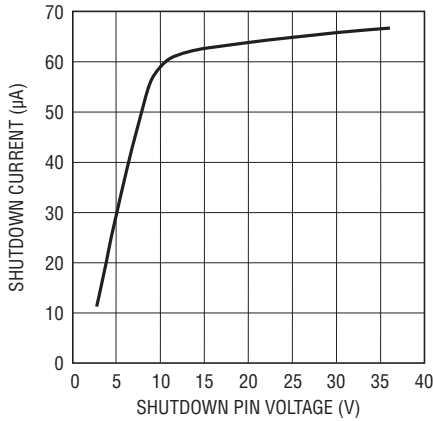
\overline{\text{SHDN}} Current vs Voltage
