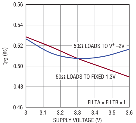
t_{PD} vs Supply Voltage and Termination Voltage
