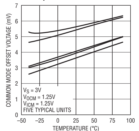
Common Mode Offset Voltage vs Temperature
