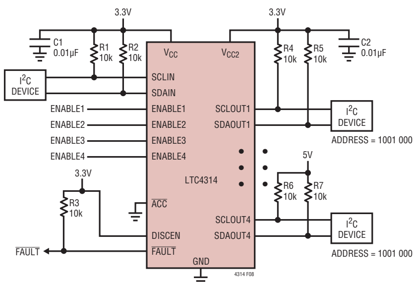
Figure 8. Nested Addressing
