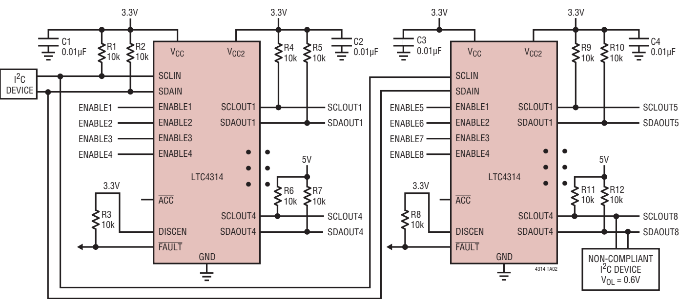
1:8 Multiplexer with Level Translation and Operation with a Non-Compliant I 2 C Device
