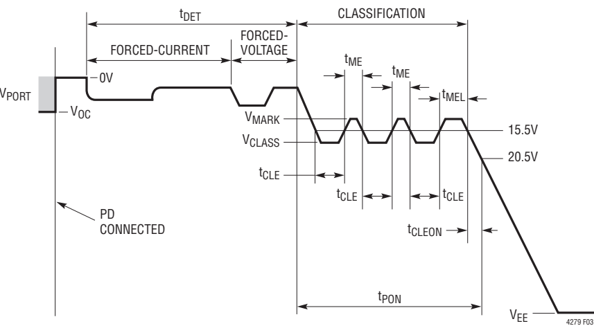
Figure 3. Detect, Three Event Class and Turn-On Timing
