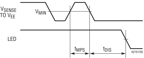
Figure 5. DC Disconnect Timing
