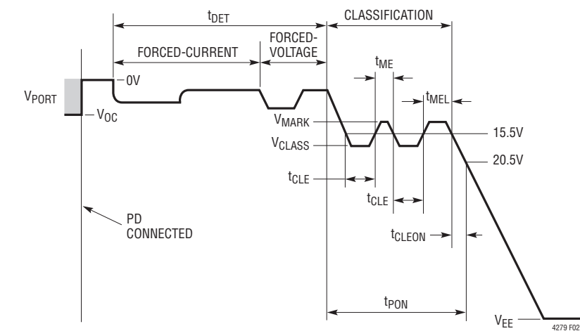
Figure 2. Detect, Two Event Class and Turn-On Timing
