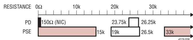
Figure 8. IEEE 802.3at Signature Resistance Ranges
