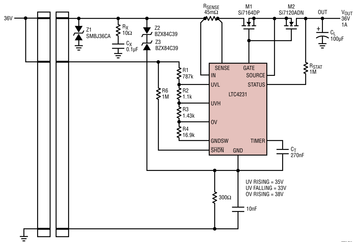
Figure 11. 36V Hot Swap Application with Reverse Protection
