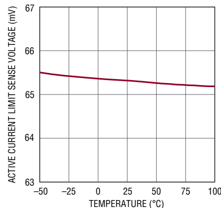
Active Current Limit Sense Voltage vs Temperature
