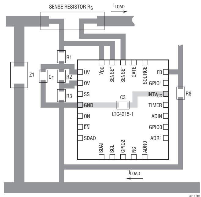
Figure 5. Recommended Layout
