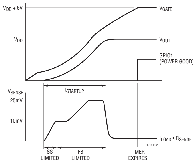
Figure 2. Power-Up Waveforms
