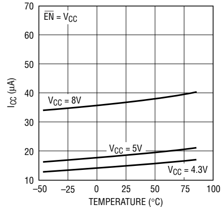
Shutdown Supply Current vs Temperature and V_{CC}
