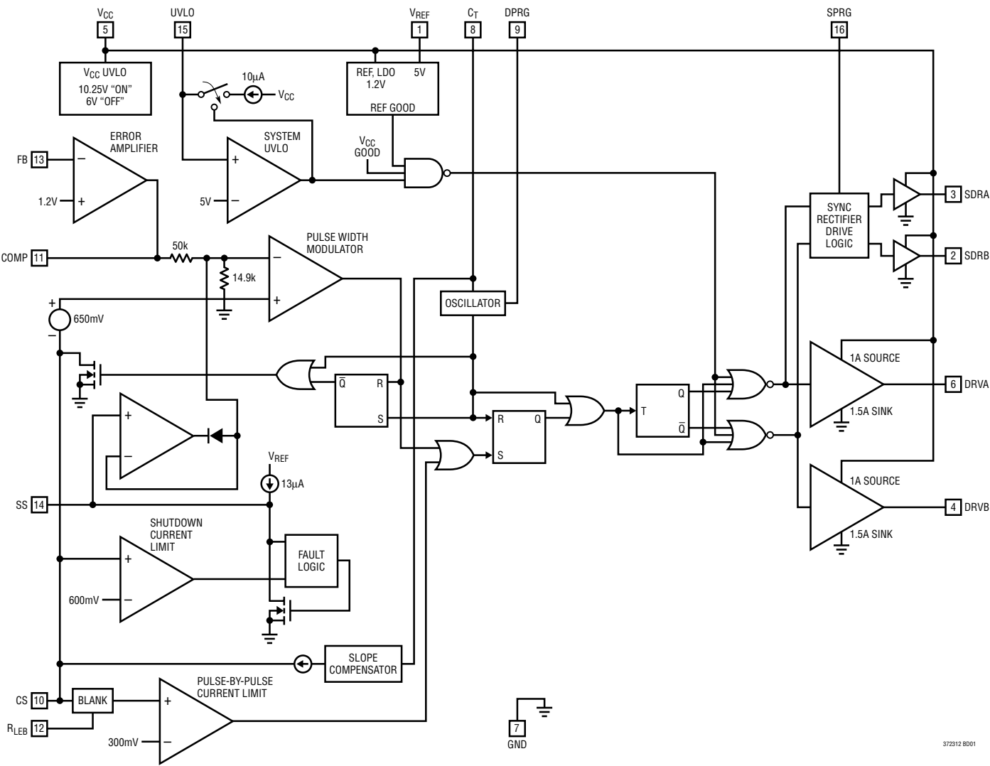
LTC3723-1 Block Diagram
