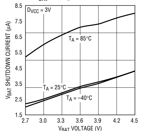
V_{BAT} Shutdown Current vs V_{BAT} Voltage
