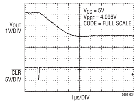
Hardware \overline{CLR} to Midscale
