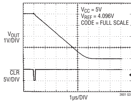
Hardware \overline{CLR} to Zero Scale
