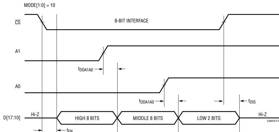
Figure 18. 8-Bit Parallel Interface Using A[1:0] Pins
