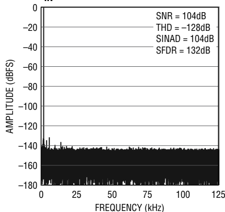
128k Point FFT f_S = 250\text{kpsps} , f_{IN} = 2\text{kHz}
