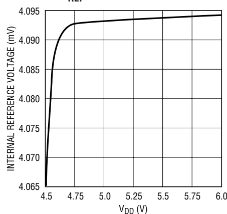
Positive Power Supply Rejection for V_{REF}
