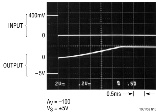
Overload Recovery
