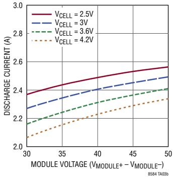
Average Flyback Output Current
