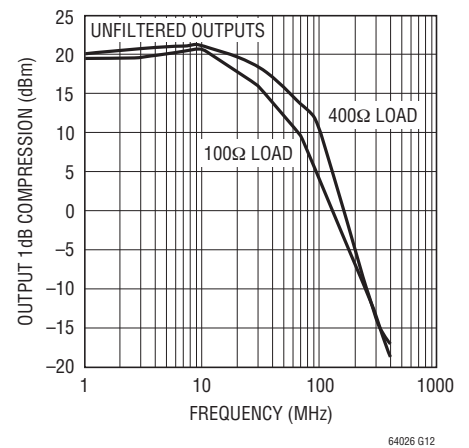
Output 1dB Compression vs Frequency
