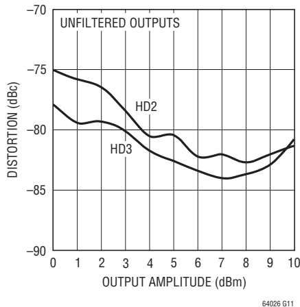
Distortion vs Output Amplitude, 20MHz Differential Input, No R_{LOAD}
