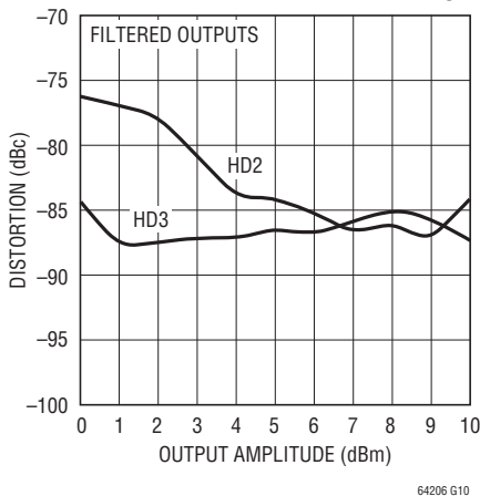
Distortion vs Output Amplitude, 20MHz Differential Input, No R_{LOAD}
