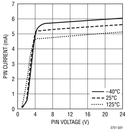
V CC Pin Current
