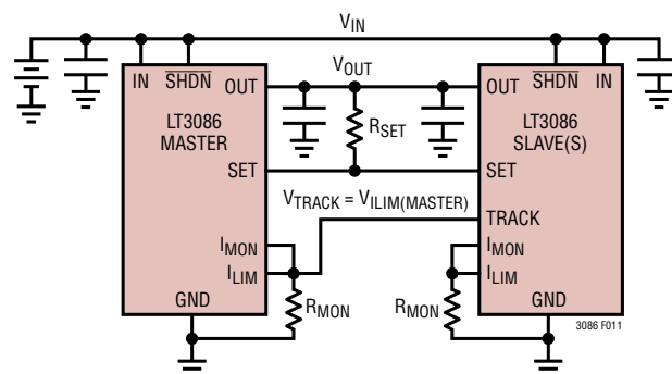
Figure 11. Master/Slave(s) Configuration for Paralleling
