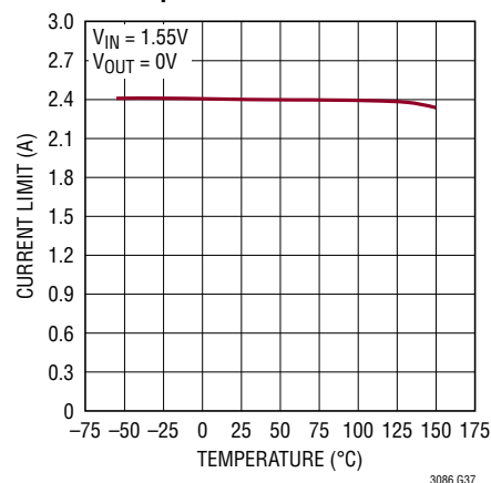
Internal Current Limit vs Temperature
