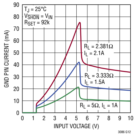
GND Pin Current, V_{OUT} = 5\text{V} (Heavy Load)
