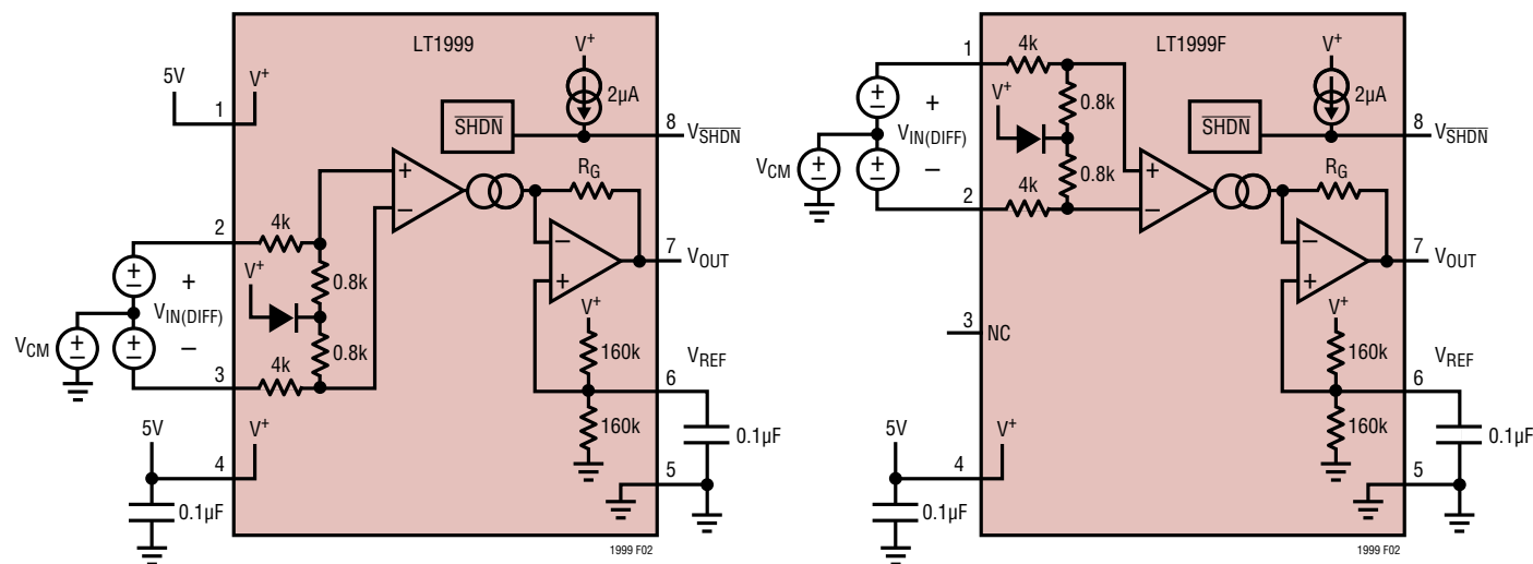
Figure 2. Test Circuit
