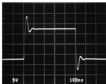
Large-Signal Transient ( G = -1 )
