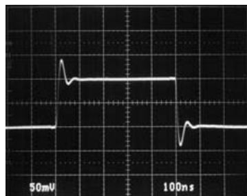
Small-Signal Transient ( G = -1 )
