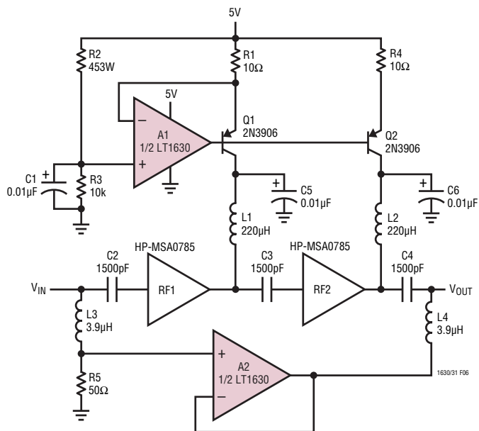
Figure 6. RF Amplifier Control Biasing and DC Restoration
