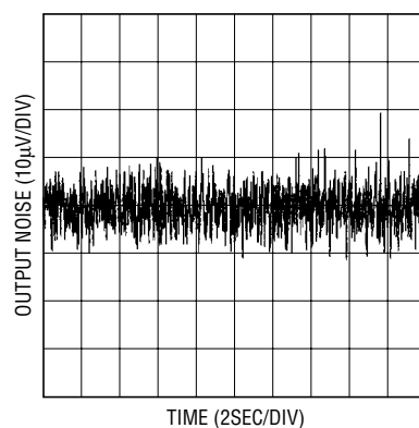
2.5V Output Noise 0.1Hz ≤ f ≤ 10Hz
