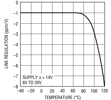
5V Line Regulation vs Temperature
