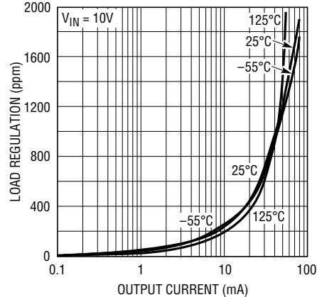
5V Load Regulation
