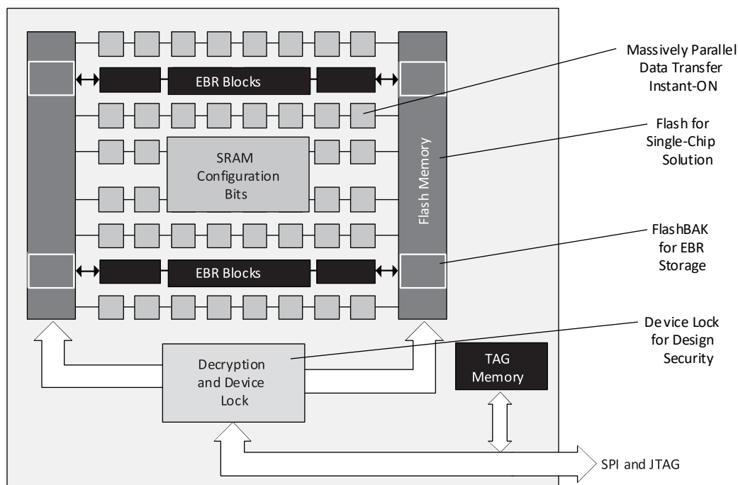
At power-up, or on user command, data is transferred from the on-chip Flash memory to the SRAM configuration cells that control the operation of the device. This is done with massively parallel buses enabling the parts to operate within microseconds of the power supplies reaching valid levels; this capability is referred to as Instant-On.
