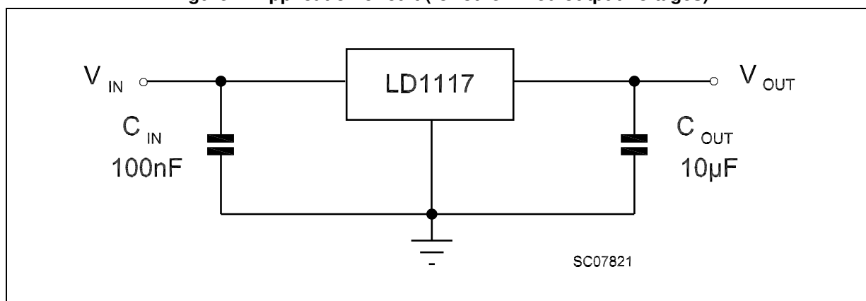
Figure 4. Application circuit (for other fixed output voltages)
