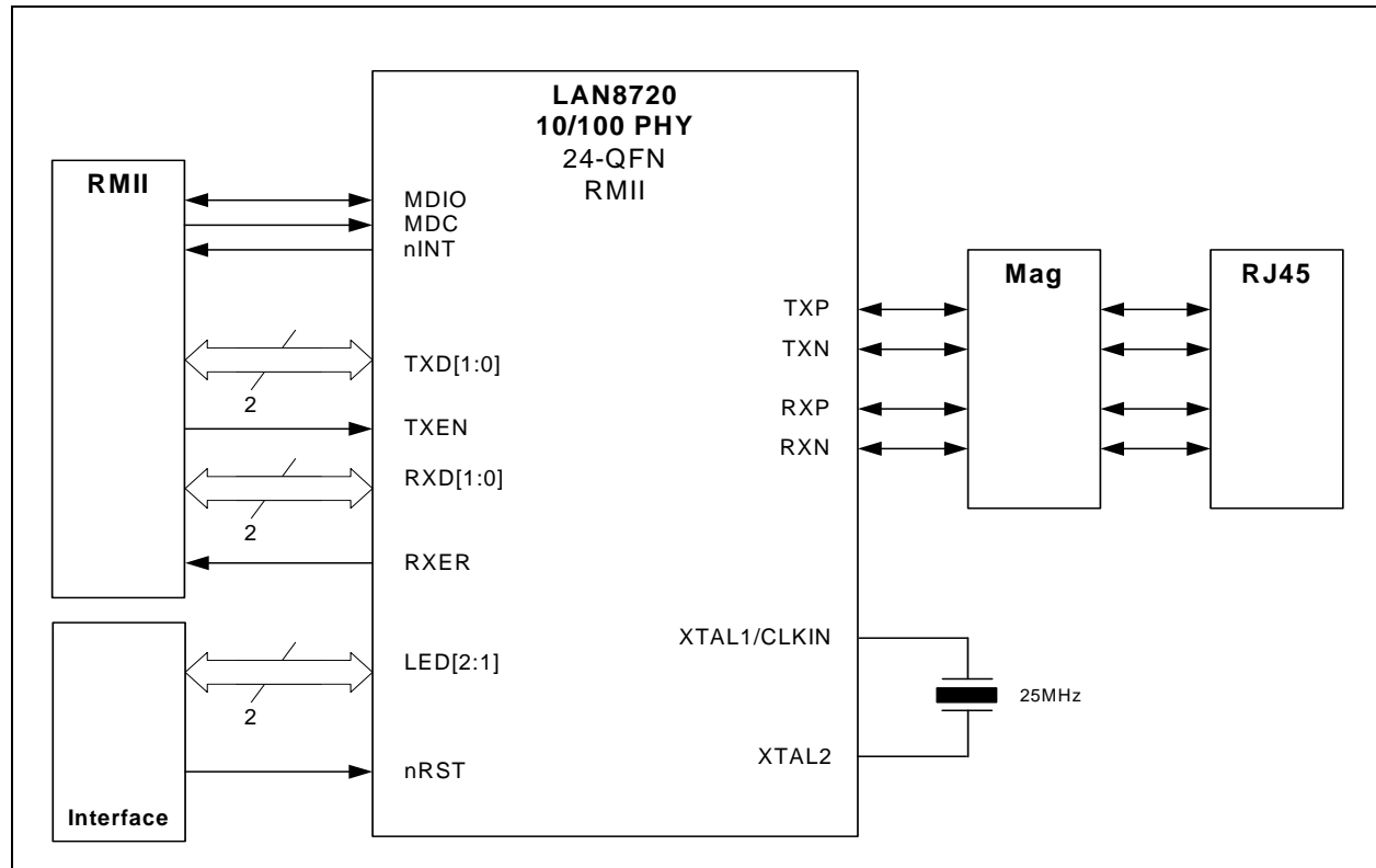
FIGURE 7-1: SIMPLIFIED APPLICATION DIAGRAM
