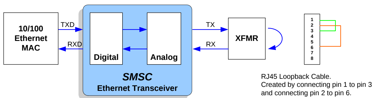
Figure 3.14 Connector Loopback Block Diagram
