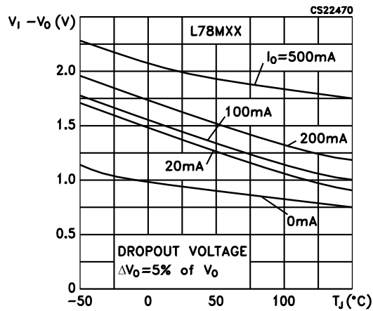
Figure 8. Dropout voltage vs junction temp.
