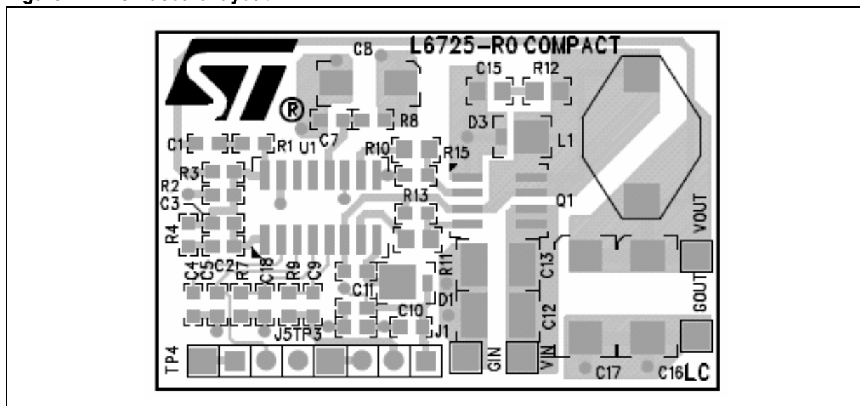
Figure 22. Demoboard layout
