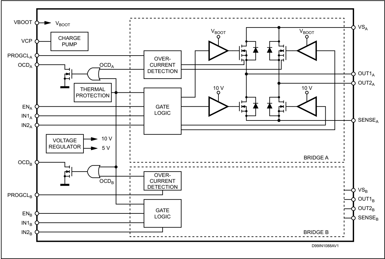
Figure 1. Block diagram
