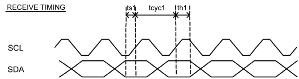
Figure 13. EEPROM Interface Input Receive Timing Diagram
