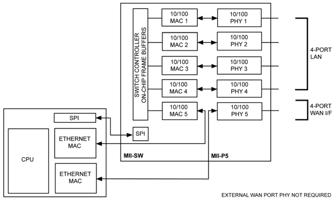
Figure 1. Broadband Gateway
