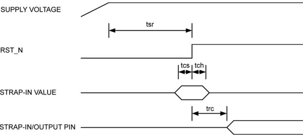
Figure 23. Reset Timing
