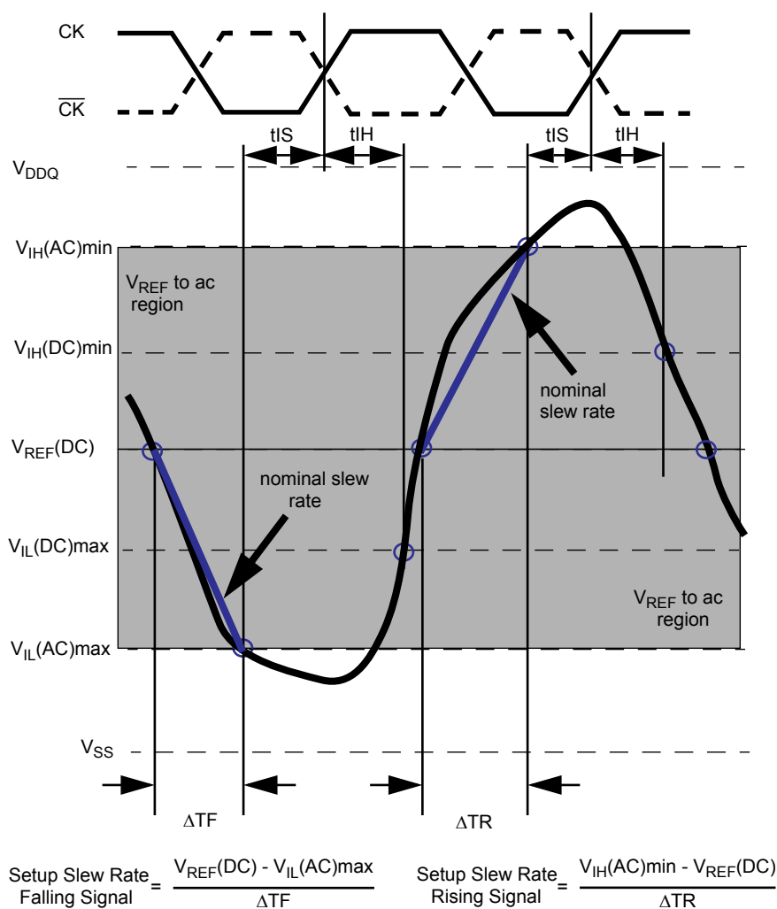
Figure 15. Illustration of nominal slew rate for t_{1S}
