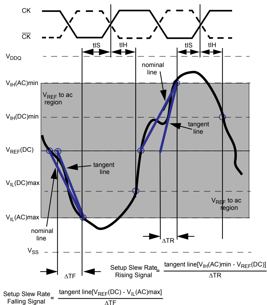
Figure 16. Illustration of tangent line for t_{\text{IS}}
